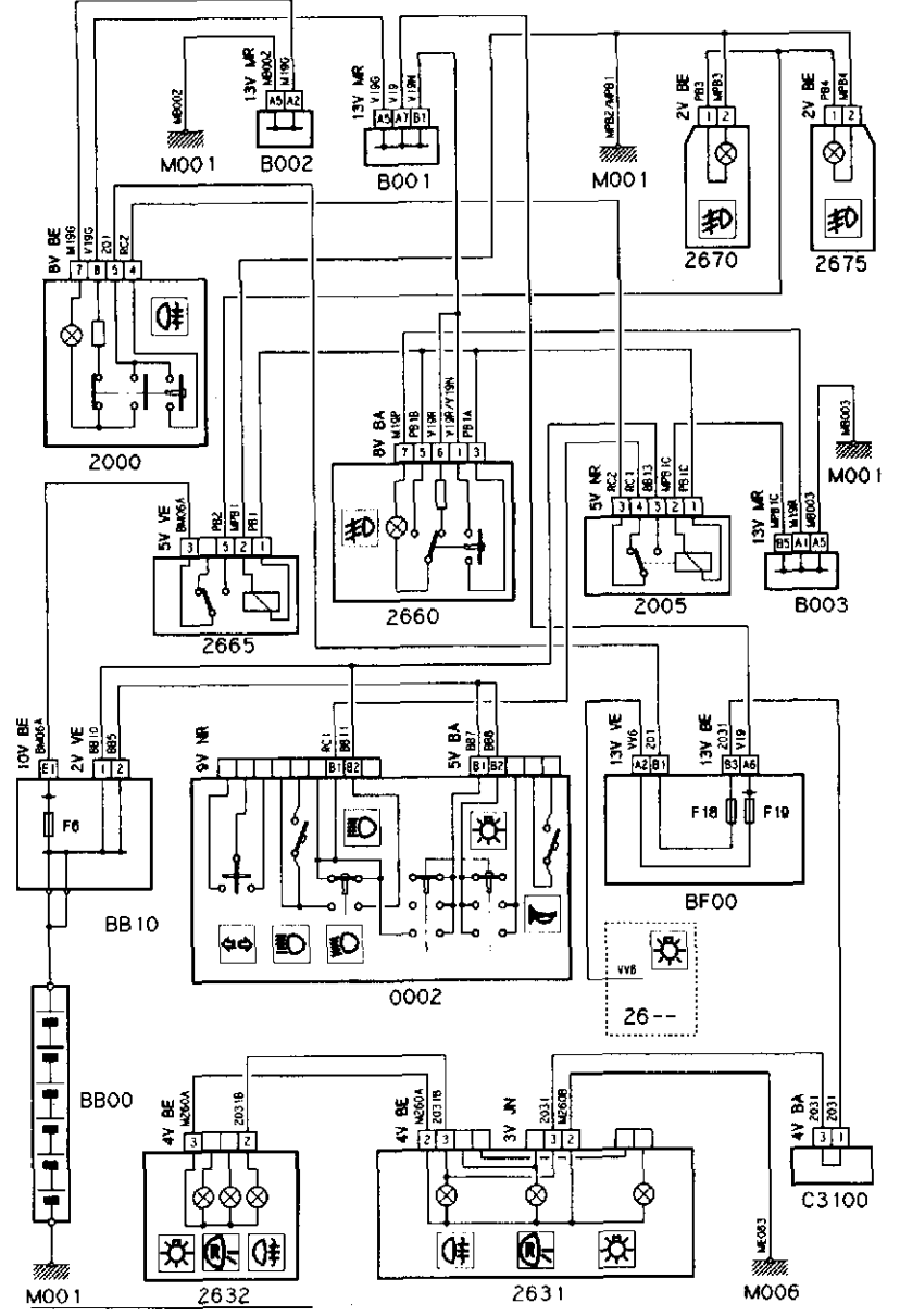
Front/rear foglights
