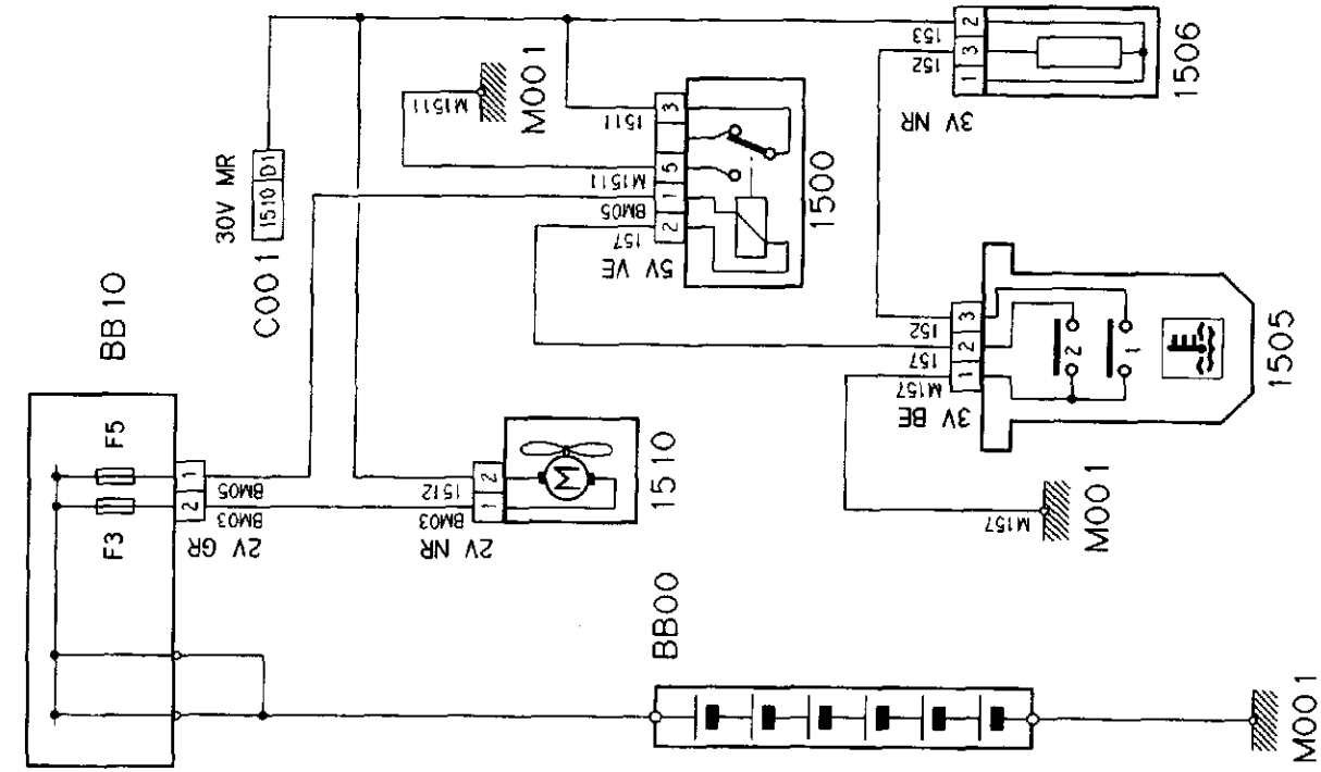
Diesel (non turbo) cooling system
