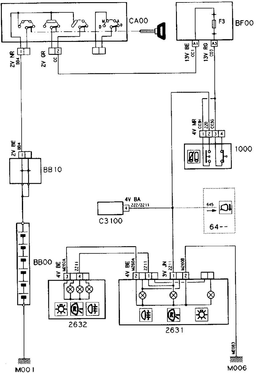
Reversing lights (automatic gearbox)
