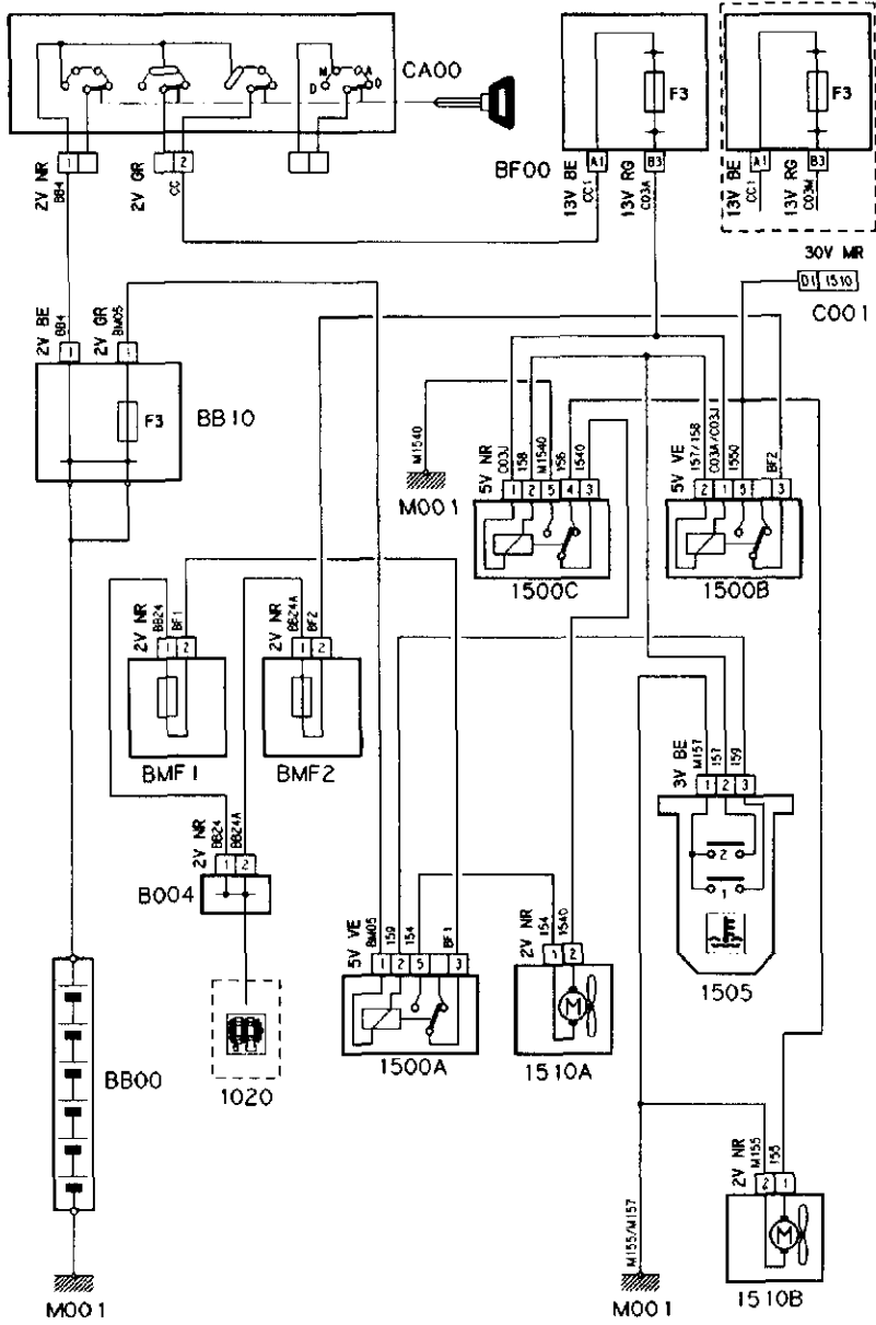
Turbo Diesel cooling system
