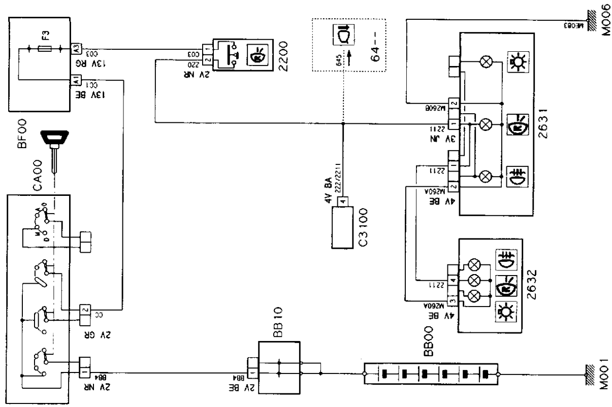
Reversing lights (manual gearbox)
