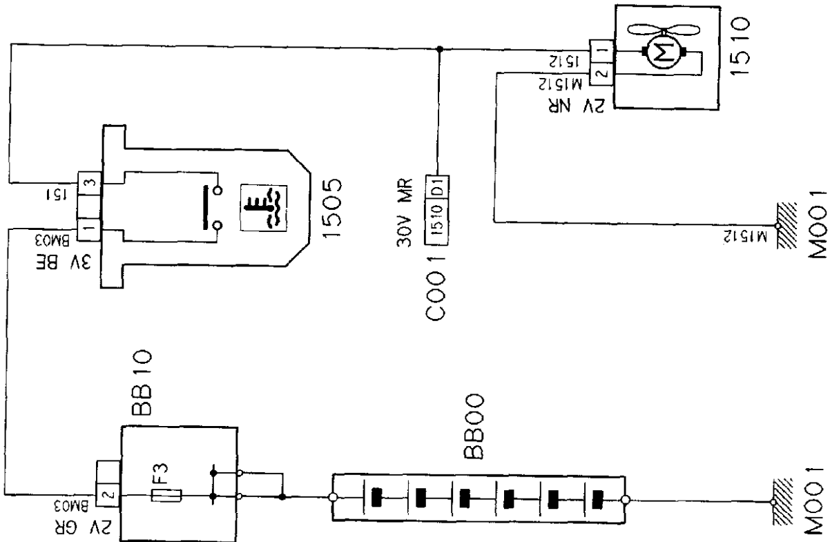
Typical XU5/XU7/XU10J2 cooling system
