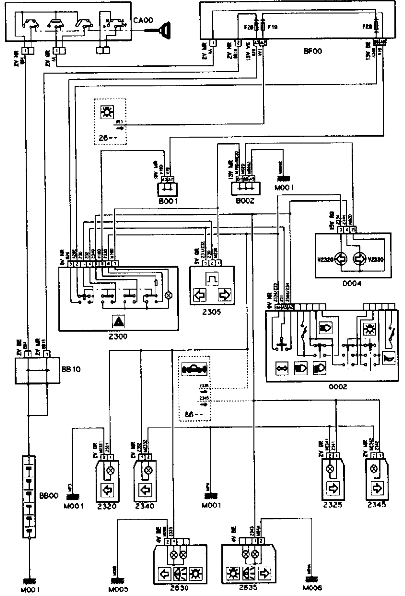
Direction indicators and hazard warning lights
